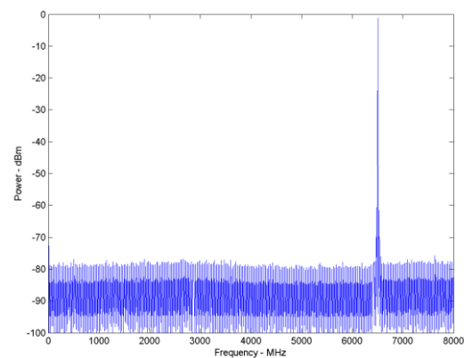
Figure 9b: 6.5GHz Broad Band Spectrum
